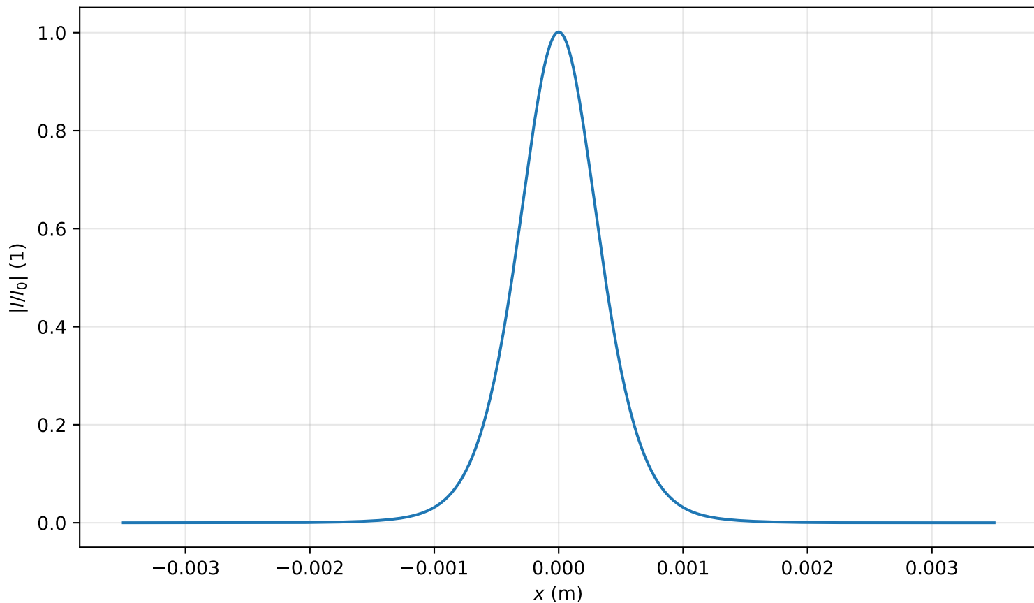
Intensity profile I(x, y = 0, z = 2.388m)/I_0 , P_{in}=0.7P_{cr} , artificial time
